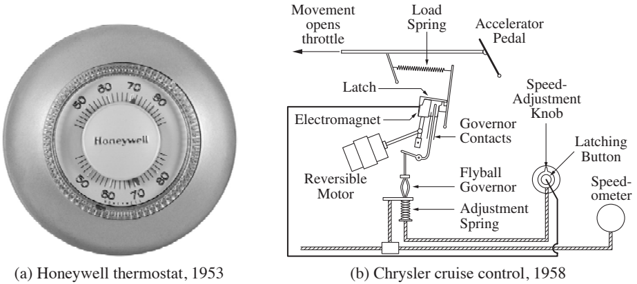
Figure 1.4: Early control devices. (a) Honeywell T87 thermostat originally introduced in 1953. The thermostat controls whether a heater is turned on by comparing the current temperature in a room to a desired value that is set using a dial. (b) Chrysler cruise control system introduced in the 1958 Chrysler Imperial [170]. A centrifugal governor is used to detect the speed of the vehicle and actuate the throttle. The reference speed is specified through an adjustment spring. (Left figure courtesy of Honeywell International, Inc.)
